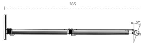
PARAFLEX® CLASSIC STANDARD ARM
